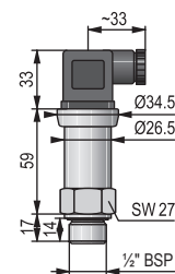
DRC-300, DEQ-300 p \leq 40 bar
