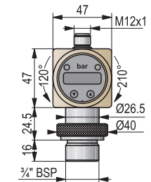
DKD-3□□□□ front view
