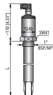
RCM / RCP-402 / 430 with M12 connection
