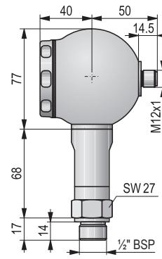
DKC-6□2-□ side view
