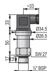
DRC-300, DEQ-300 p \geq 60 bar
