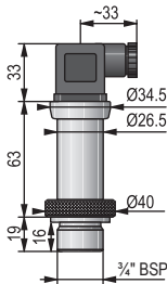
DRD-6□2-□ for SIL and SIL / Ex ia versions
