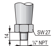
DKG-500□□□□ side view
