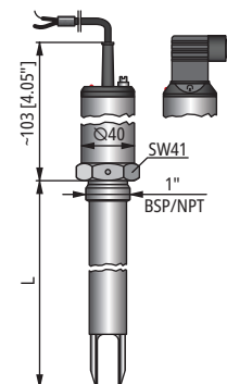
RCM / RCP-402 / with DIN connection or integrated cable
