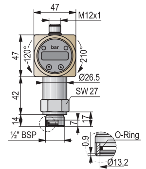
DKC-3□□□□ front view
