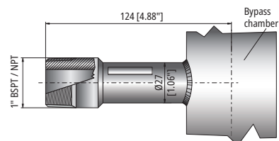
MOX-000-0 (¾" BSPT), MOY-000-0 (¾" NPT) Threaded connection
